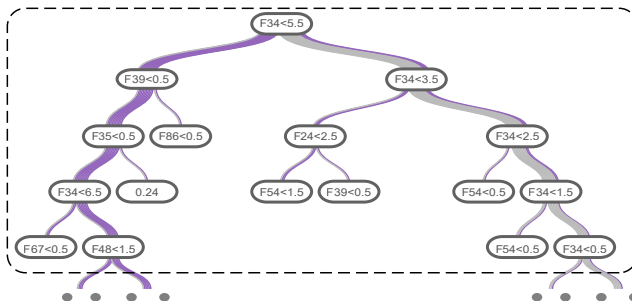
Fig. 5. Decision tree for the violet class in iteration 1. Feature F34 at the top layer can separate most instances of the violet class from the others.
